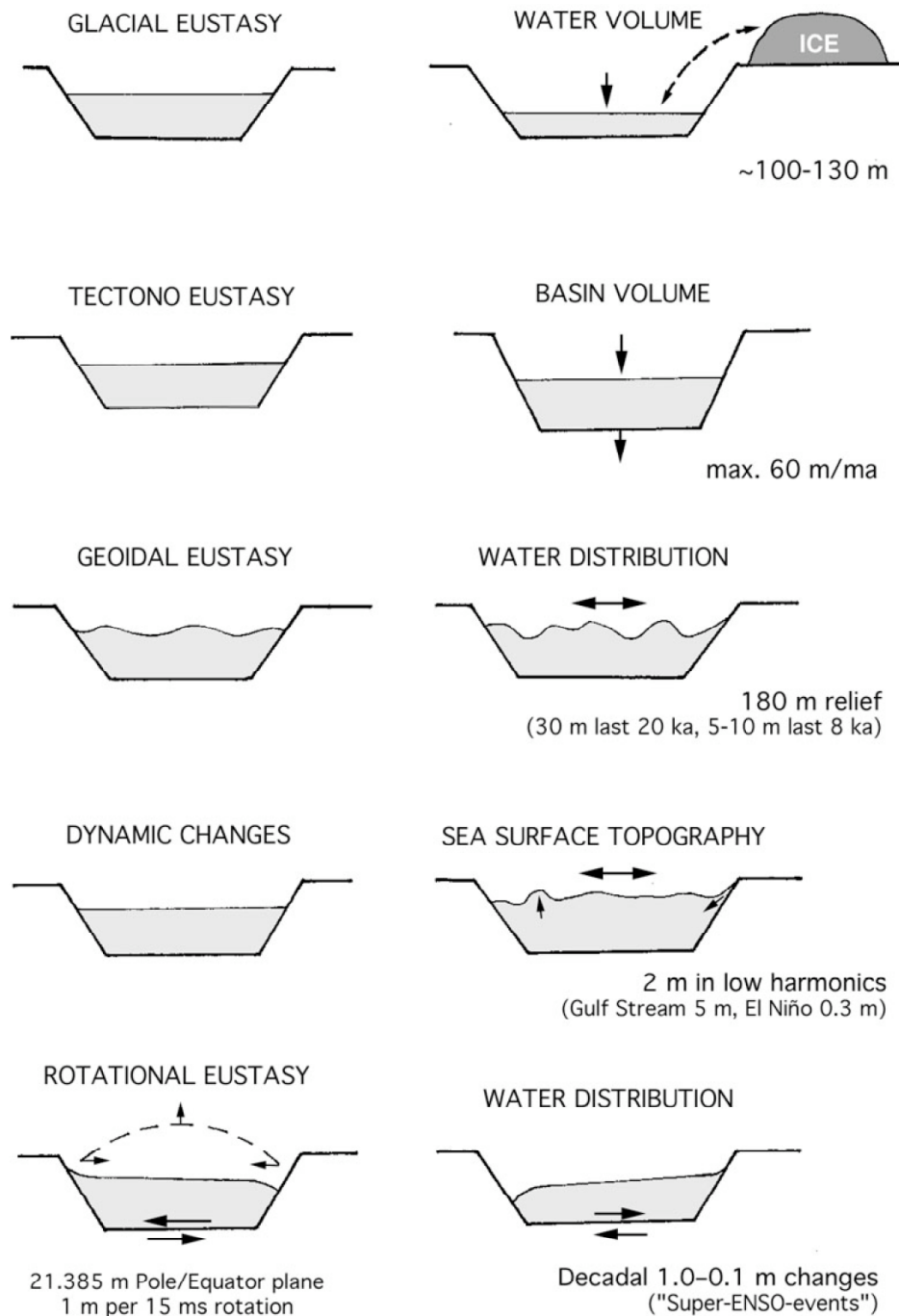
Fig. 5 - Main eustatic variables with some quantification added. The glacial eustasy in the Quaternary has a sea level range of about 100-130 m. Tectono - eustasy is a very slow process, of negligible significance in the Holocene, with a maximum rate of 0.06 mm/year.
