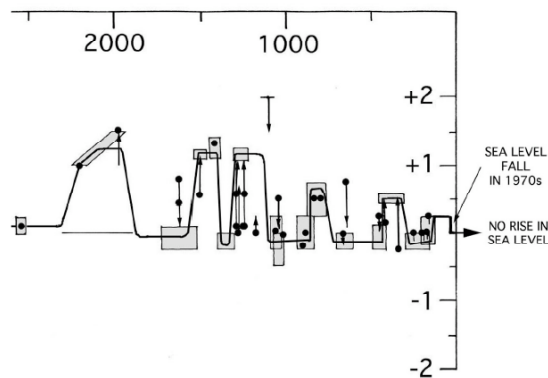
Fig. 4 - The sea level record of the past 2600 years from the Maldives including a significant sea level fall in the 1970s and a lack of signs of any ongoing rise (from MÖRNER, 2007b).
