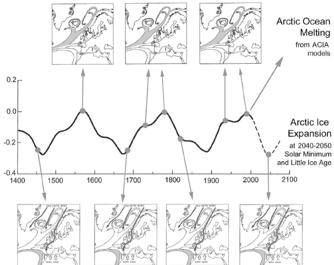
Fig. 2 - The main Solar cycle in the last 600 years with observed ocean circulation pattern at maxima and minima, and the expected extension into the future (from MÖRNER, 2005a). At Solar minima NW Europe, the North Atlantic and the Arctic have experienced cold phases known as “Little Ice Ages”. By year 2040-2050, a new Solar Minimum is to be expected, and with a new cold phase over the Arctic and NW Europe.
